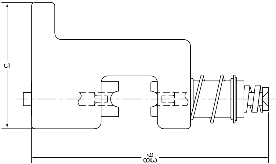
SIDE VIEW, OPEN UNIT
